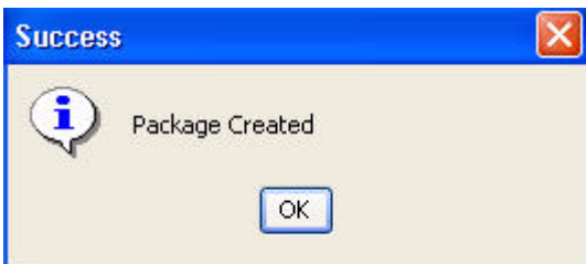
Figure 6-6 Success Message
