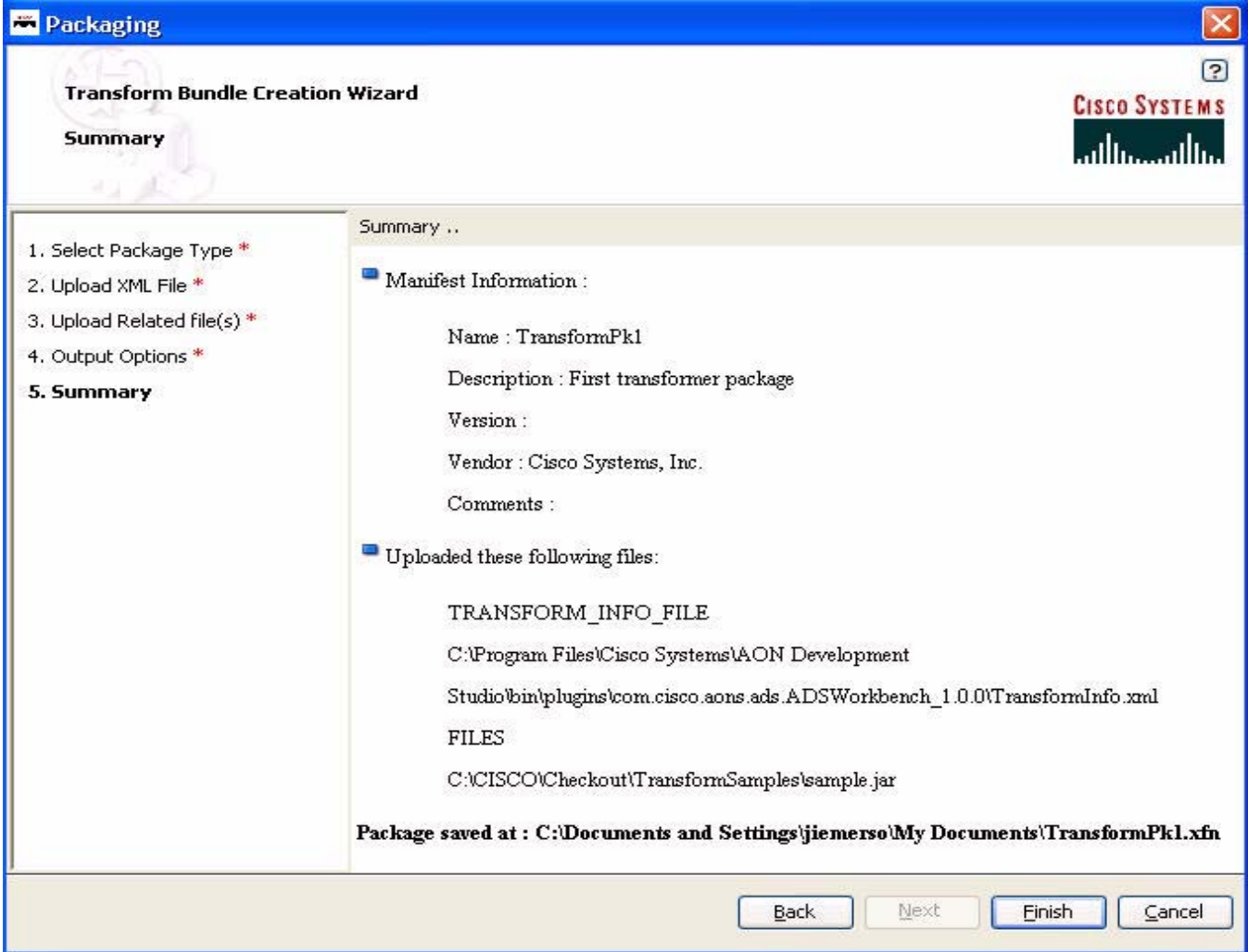
Figure 6-5 Summary
