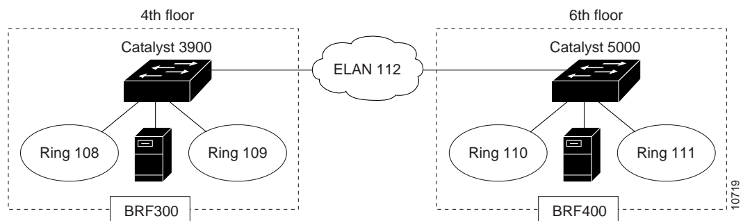
Figure 10-6 Resulting Network Configuration
