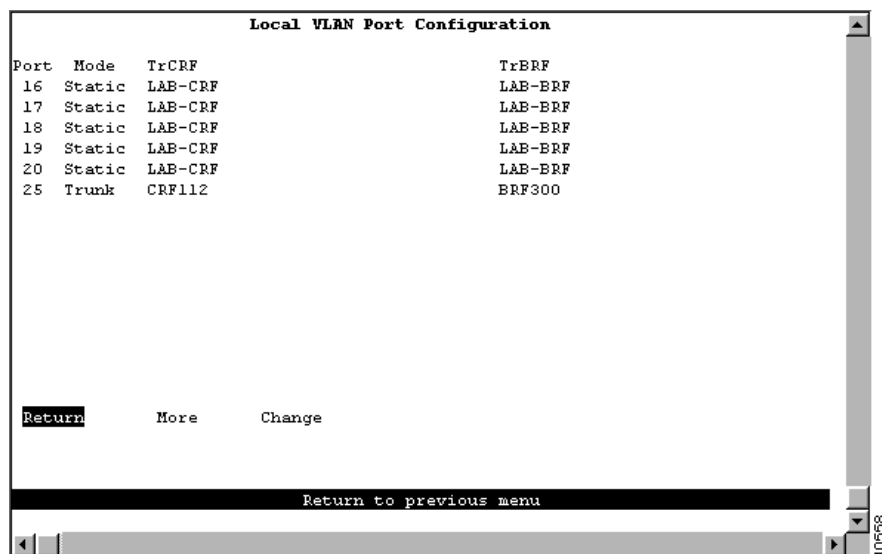
Figure 10-3 Local VLAN Port Configuration Panel
