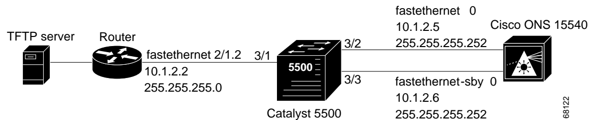
Figure 2 Example Network with TFTP Server, Router, Catalyst 5500, Cisco ONS 15540, and VLAN Trunk
