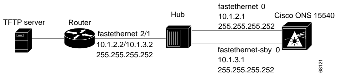
Figure 1 Example Network with TFTP Server, Router, Hub, and Cisco ONS 15540
