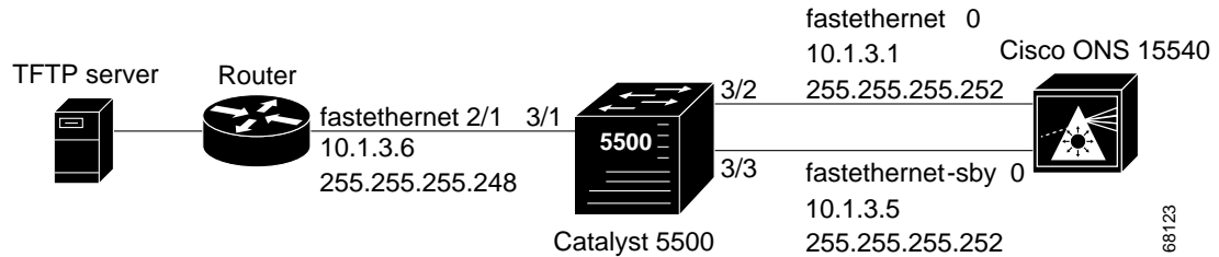
Figure 3 Example Network with TFTP Server, Router, Catalyst 5500, Cisco ONS 15540, and VLAN
