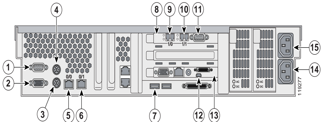
Figure 2 Rear Panel
