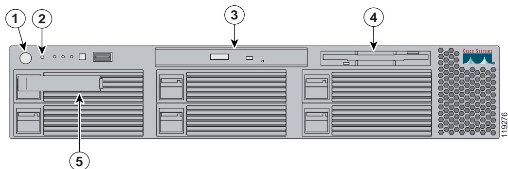
Figure 1 Front Panel
