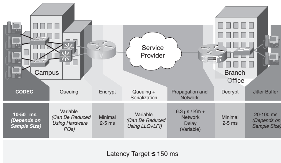
Figure 6-7 IPsec Encryption/Decryption Incremental Delays
