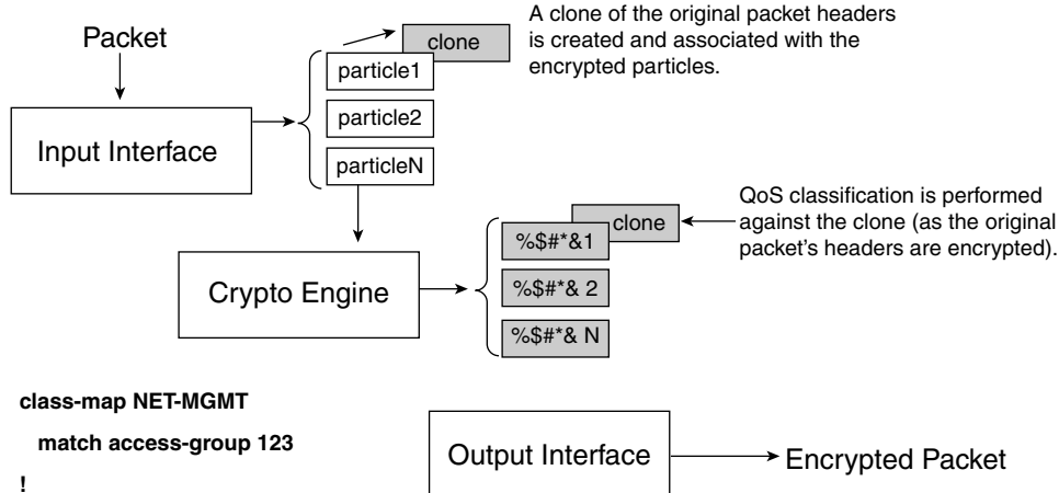
Figure 6-10 QoS Pre-Classify Feature Operation
